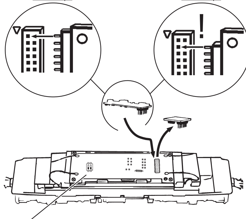
Decoder 22-pin
